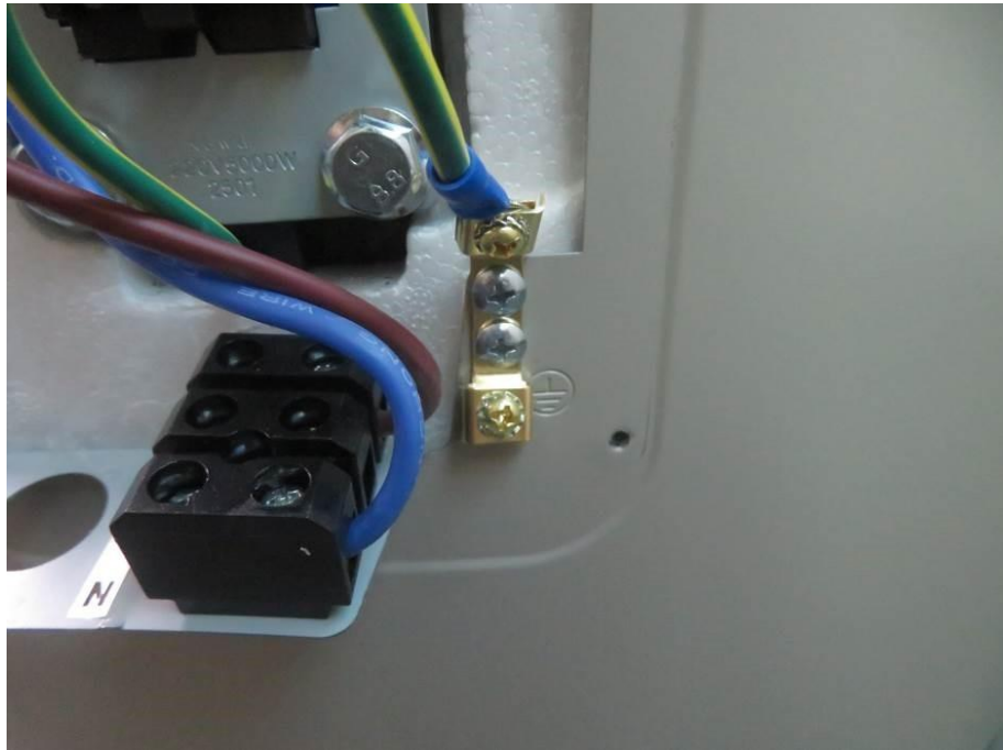
Fig. 3 – Internal view
