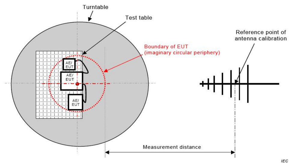
Figure C.1 – Measurement distance
