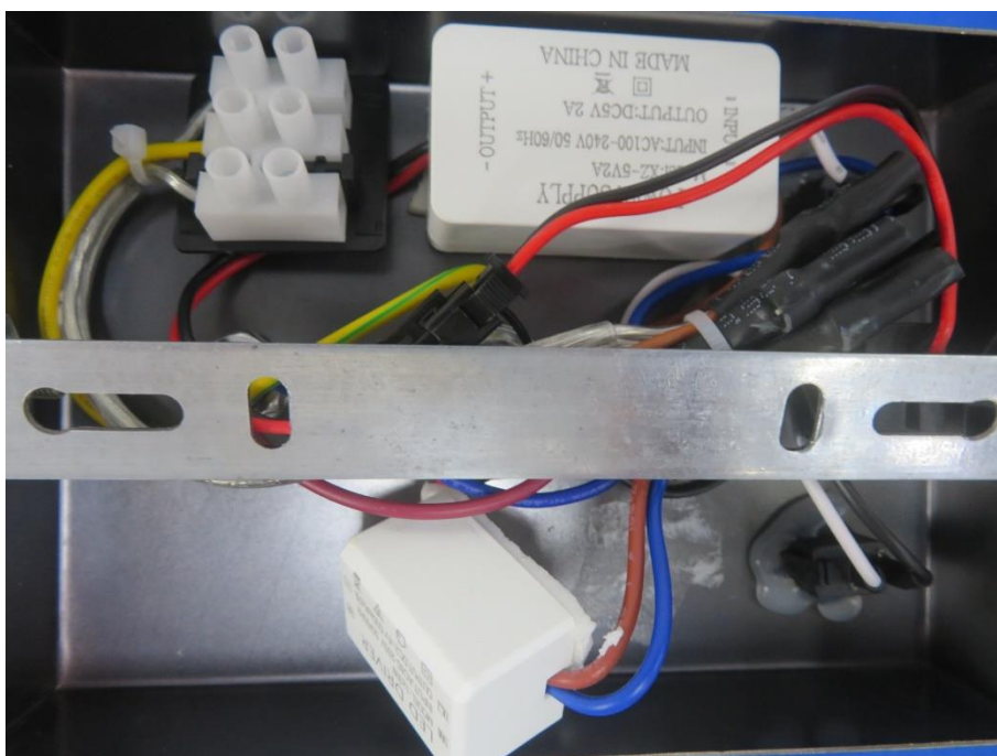
Fig. 3 (Model name: A2581AP-2AB)
