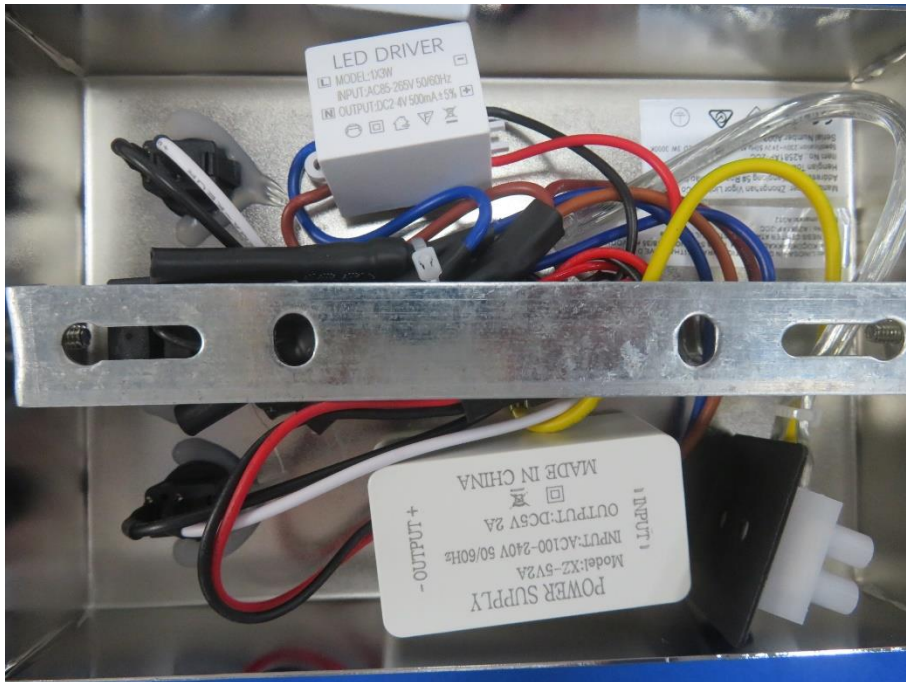
Fig. 6 (Model name: A2581AP-2CC)
