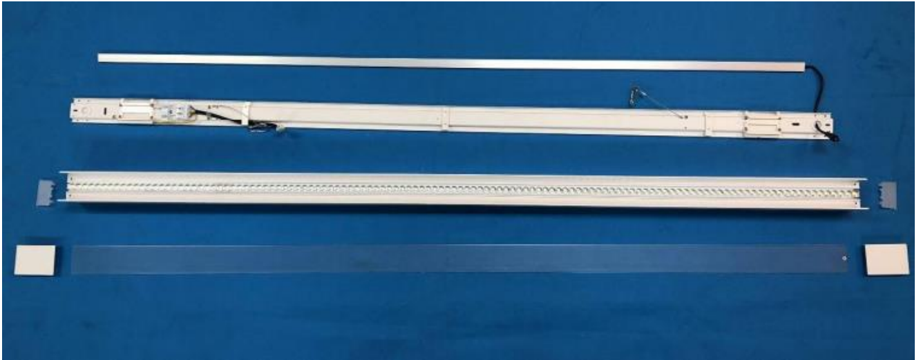
Fig.3:Internal view for all models, exploded view (Representative model DB66D-1500-49W-DO)
