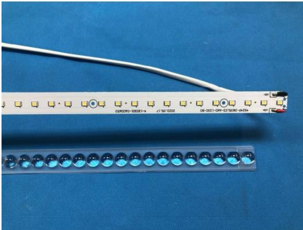
Fig.13:LED module(down) view for all models
