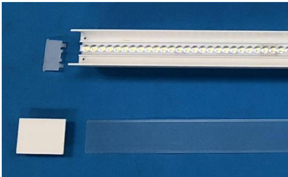
Fig.12:LED module(down) view for all models
