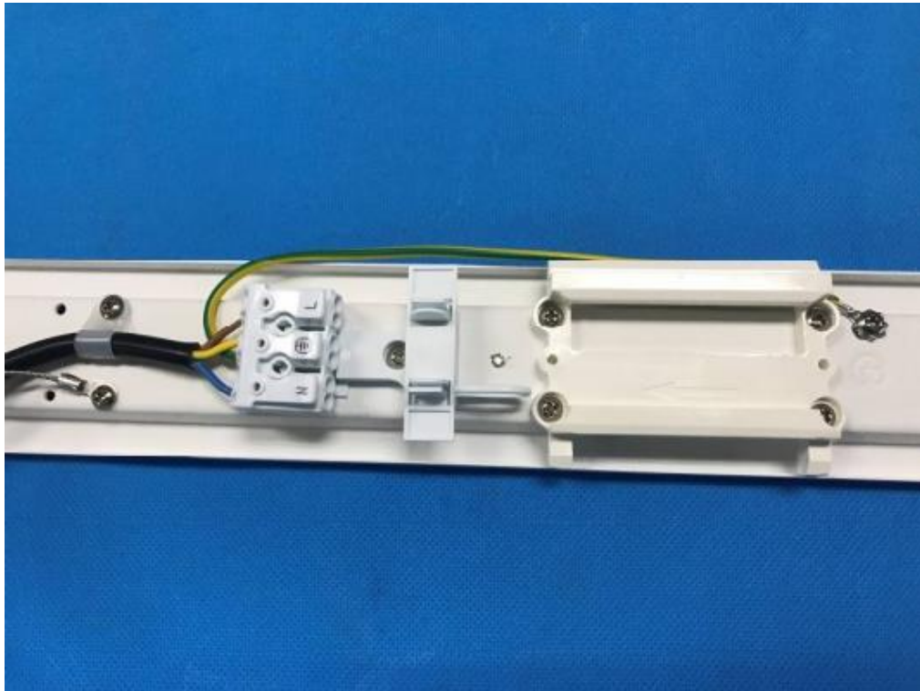
Fig.5:Terminal block view for all models
