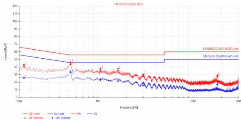
Suspected List
