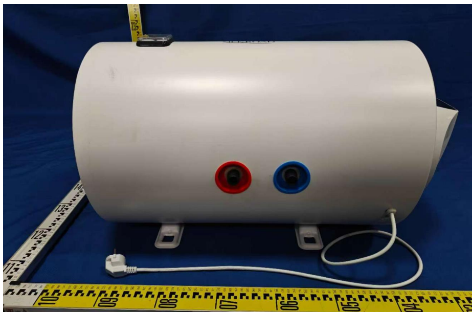
Fig.8 of H12 series: NRJ50VLA12H
